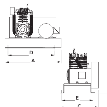
Simplex base-mount w/optional starter
