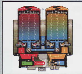
EXTENDED LIFE Mounted desiccant dryer to eliminate moisture and contaminants, - 40° F Dew Point
