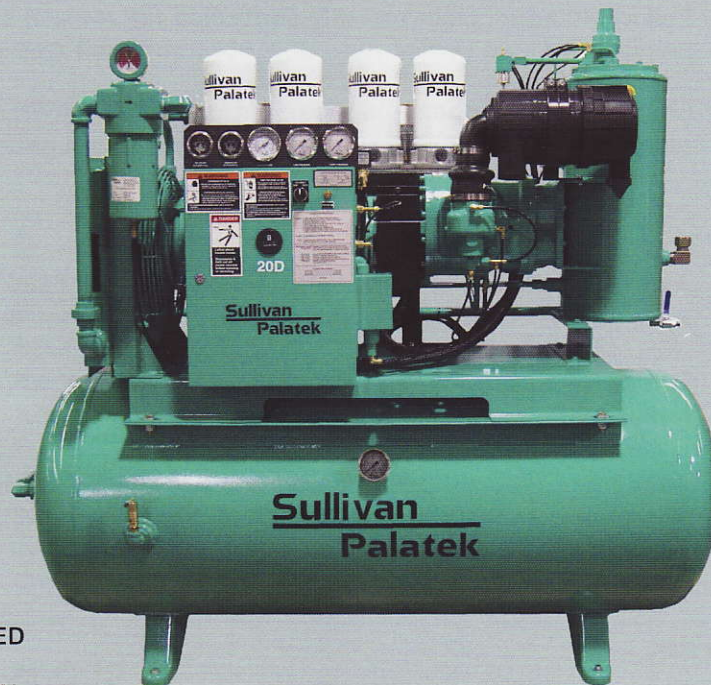
EXTENDED LIFE Mounted desiccant dryer to eliminate moisture and contaminants, - 40° F Dew Point
